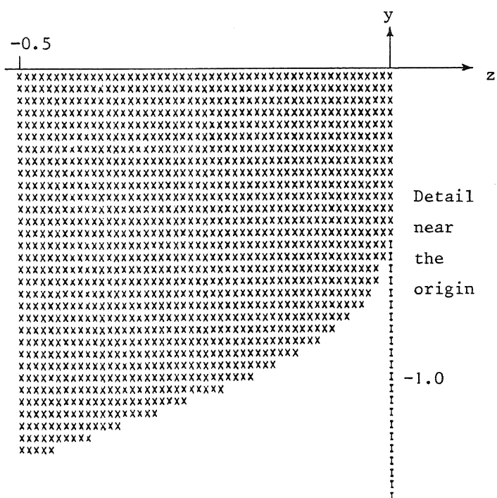
Figure 4.4 k=5
