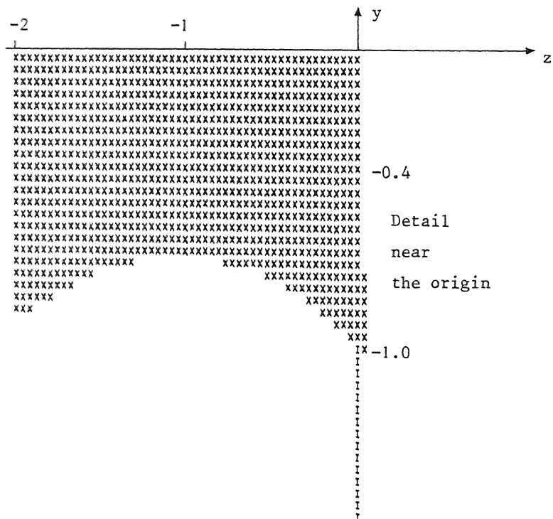
Figure 4.5 k=6
