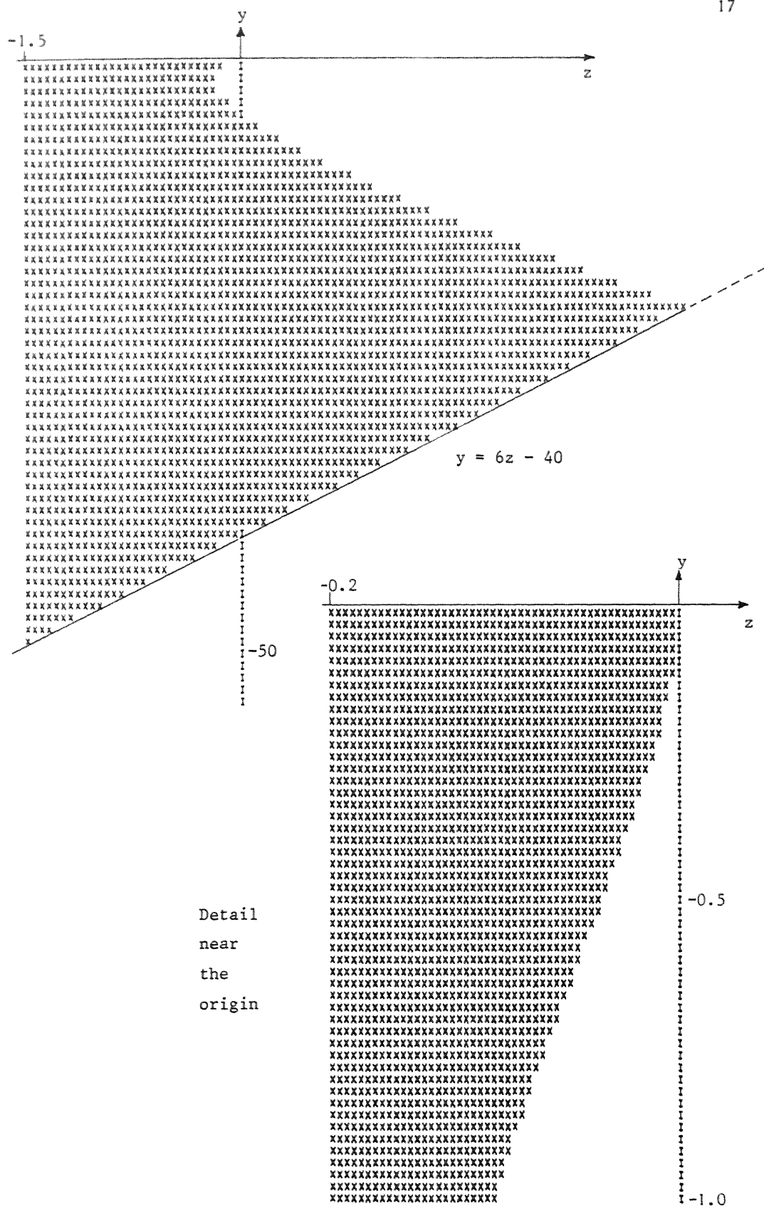
Figure 4.2 k=3
