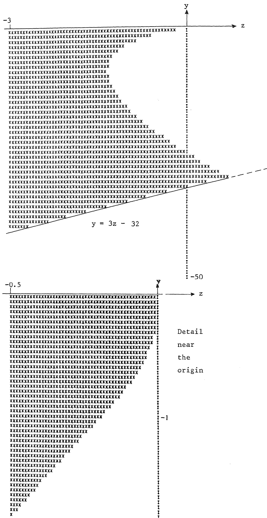
Figure 4.3 k=4
